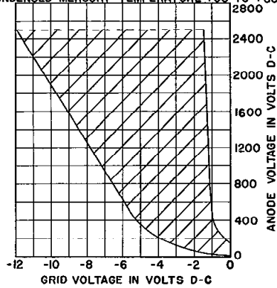
TYPICAL CONTROL CHARACTERISTICS. SHADED AREA SHOWS RANGE OF CHARACTERISTICS, CONDENSED-MERCURY TEMPERATURE +30^{\circ} TO +80^{\circ} C.
