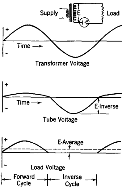
FIG. 21. Simplified chart of the voltage relations in a half-wave rectifier with a resistance load and no filter.
