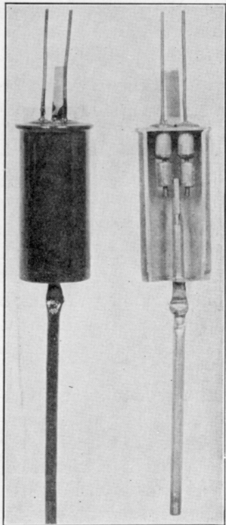
FIG. 83. A single-pole, double-throw vacuum switch.
