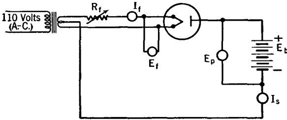
FIG. 10. Circuit for measuring the emission of a high-vacuum tube.
