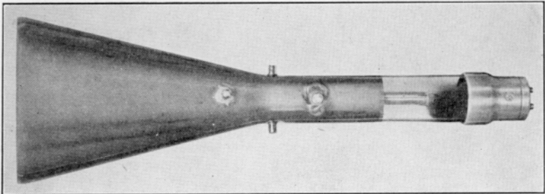
FIG. 82. A cathode-ray oscillograph tube.
