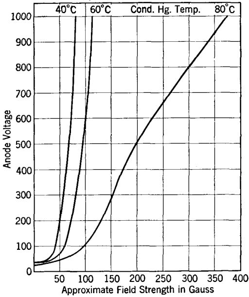
FIG. 61. A typical set of magnetic-control curves for a three-electrode, mercury-vapor tube. These curves show the relation between the transverse magnetic field intensity and the anode voltage required for breakdown. The data for these curves were taken with the control-grid voltage held at zero.
