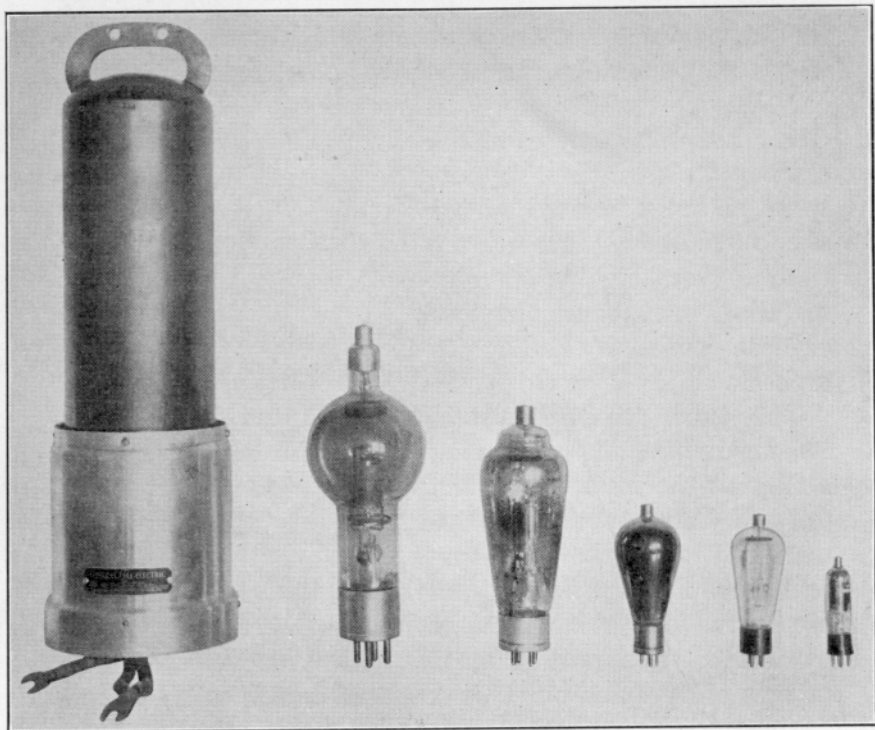
FIG. 52. A group of two-electrode, mercury-vapor-filled tubes. The average current rating, in amperes, of these tubes is: (from left to right) 100A., 12.5A., 6.4A., 2.5A., 0.5A., 0.125A.
