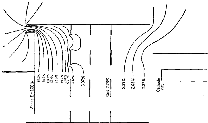
Fig. 57. The potential distribution in a "positive-grid" tube for a combination of electrode voltages which would just cause breakdown.
