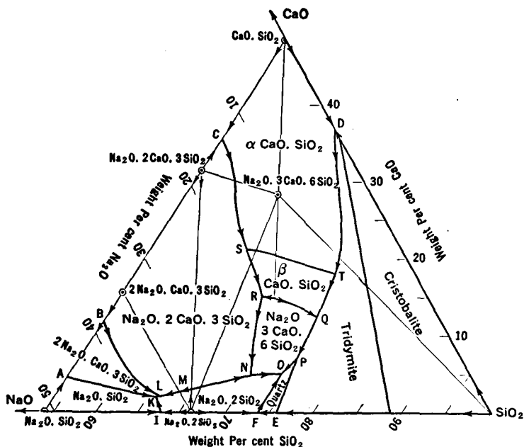
Fig. 17.8. Phase equilibrium diagram of the ternary system Na 2 O-SiO 2 -CaO-SiO 2 . Composition is expressed in weight per cent of Na 2 O, CaO and SiO 2 . After Morey and Bowen. 6 (Courtesy British Society of Glass Technology.)
