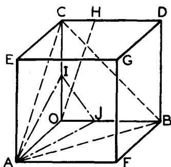
Fig. 7.4. Directions and planes in cubic lattice. Direction OA , (100) ; Direction OD , (011) ; Direction OG , (111) ; Direction OH , (01\bar{3}) ; Plane AEGF , (100) ; Plane ABDE , (110) ; Plane ABC , (111) ; Plane AIJ , (132) . (By permission from "Applied X-Rays" by G. L. Clark. Copyright 1940. McGraw-Hill Book Company, Inc.)
