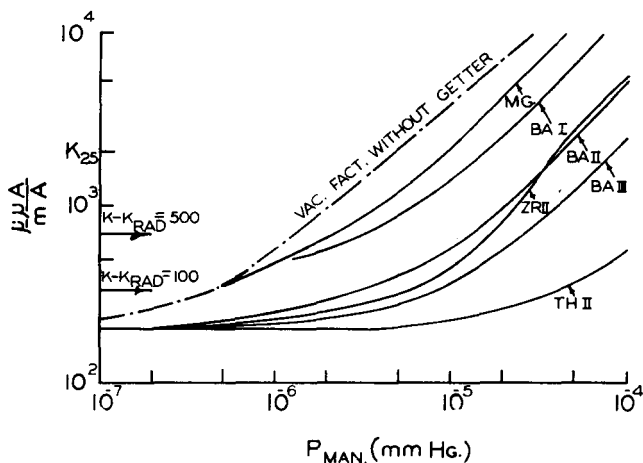
Fig. 18.1. Vacuum factor K in \mu\mu\text{A}/\text{mA} as a function of manifold pressure ( p_{\text{man}} ) for different getters. After S. Wagener. 18 (Courtesy The Institute of Physics, London, S.W. 1, England.)
