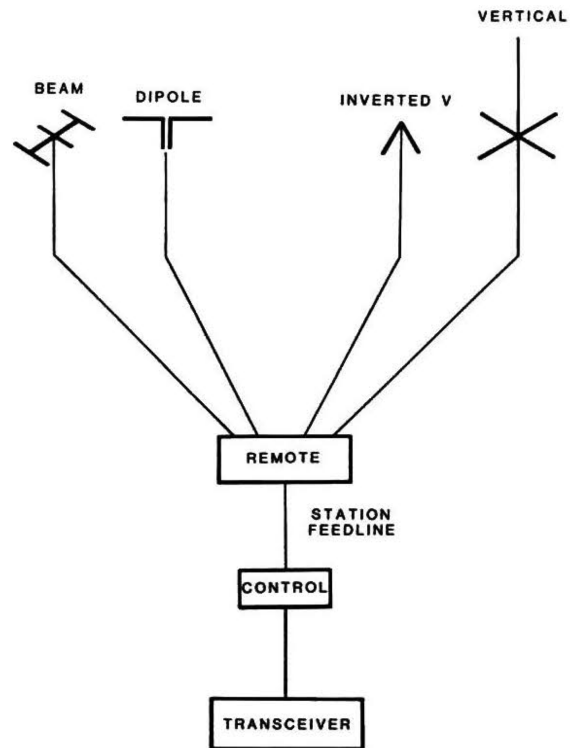
BLOCK DIAGRAM
