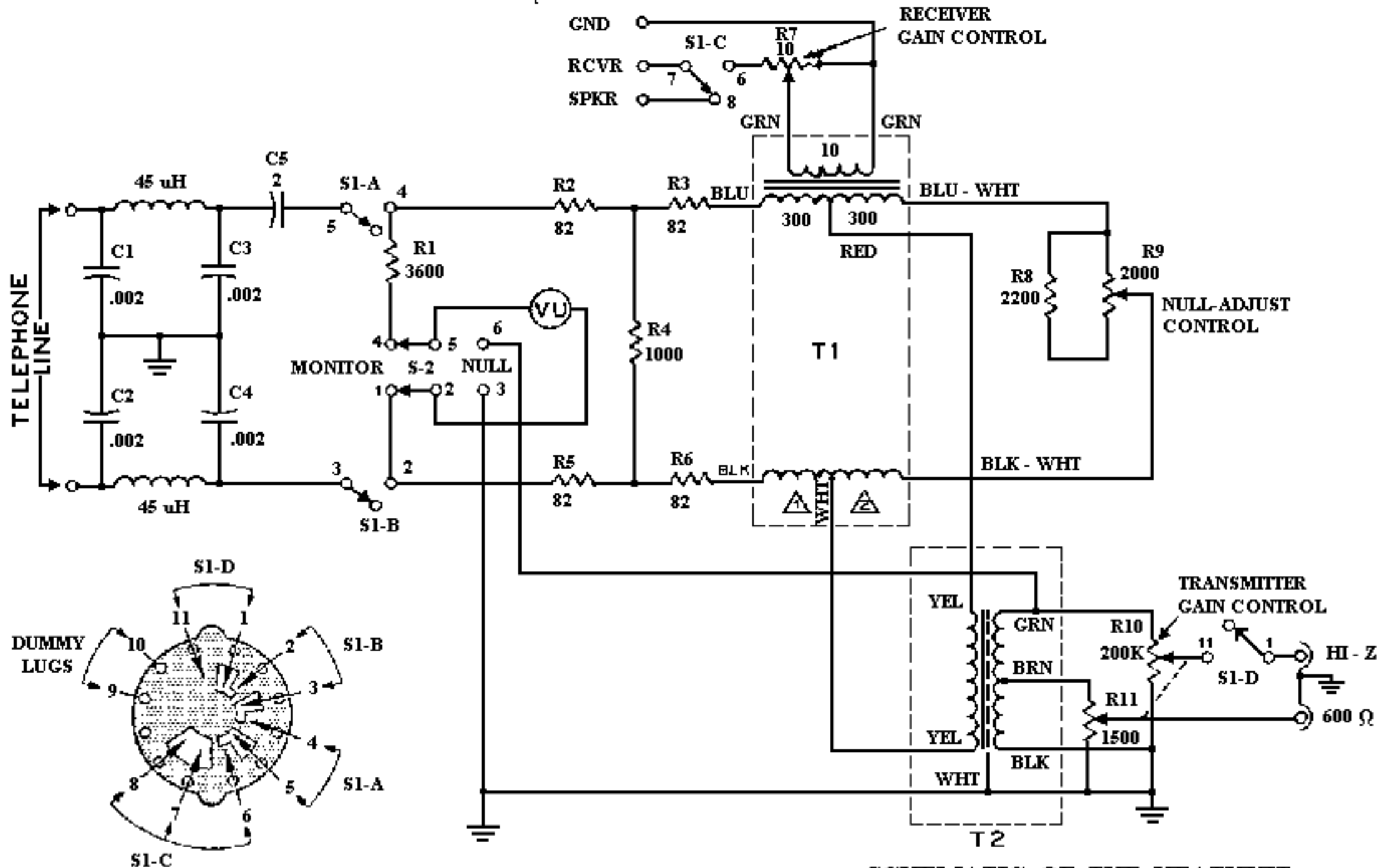
SCHMATIC OF THE HEATHKIT HYBRID PHONE PATCH MODEL HD - 15
