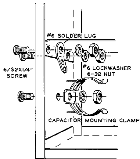
Detail 14B
