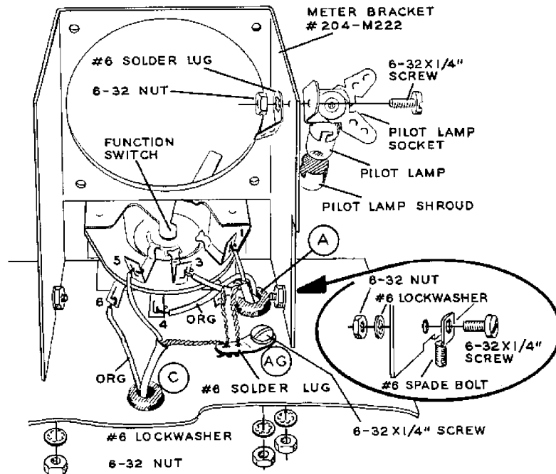
Detail 18A
