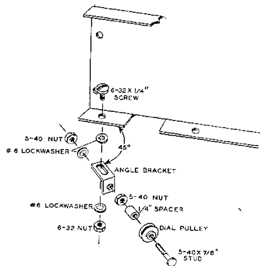
Detail 14F
