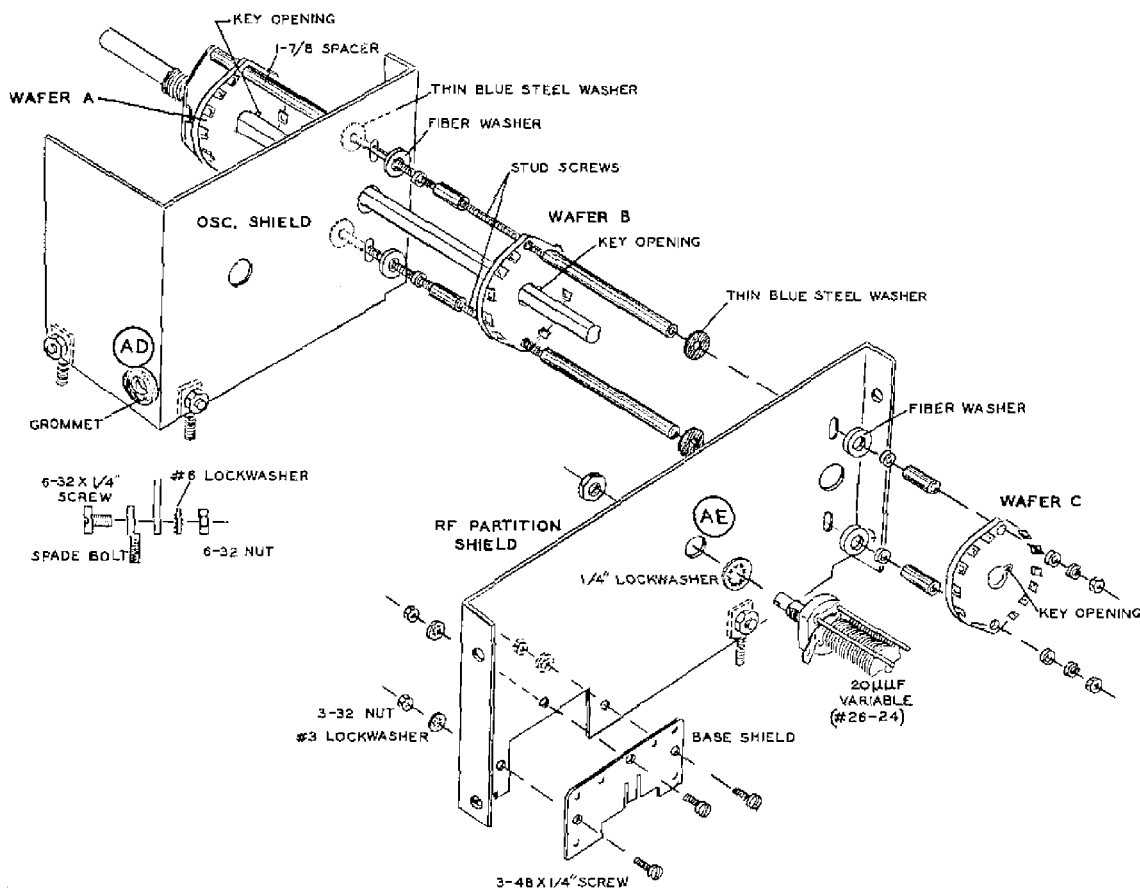
Detail 8A
