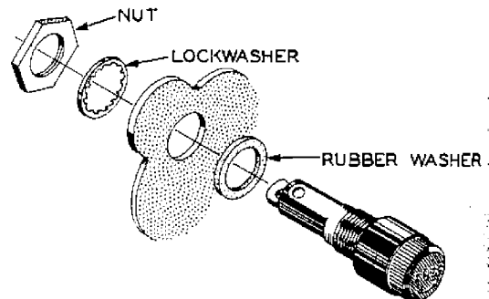
Detail 14C
