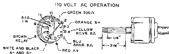
Detail 19A
