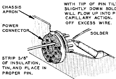
Detail 14G
