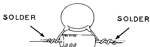
Pictorial 5
