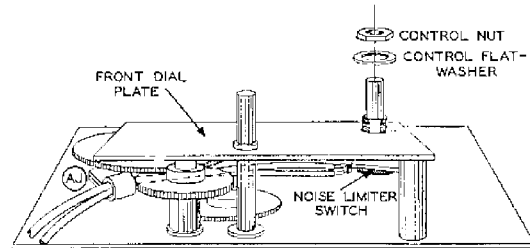
Pictorial 12
