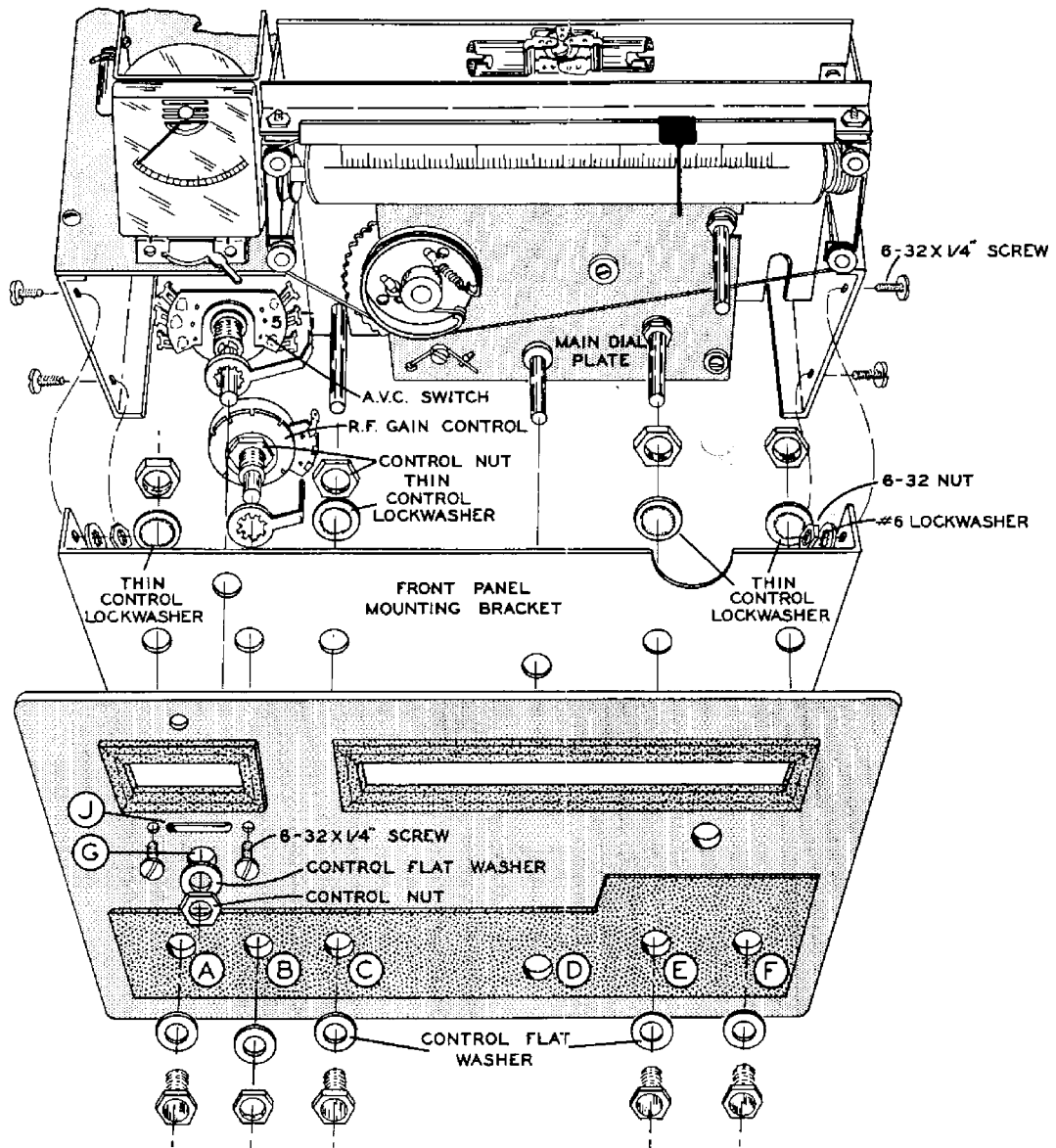
Pictorial 16
