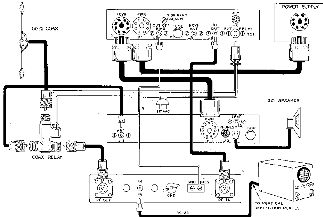
Pictorial 23
