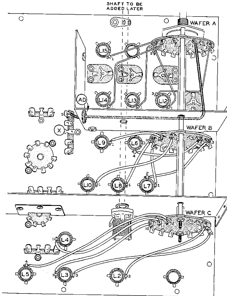
Pictorial 10
