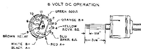
Detail 19B
