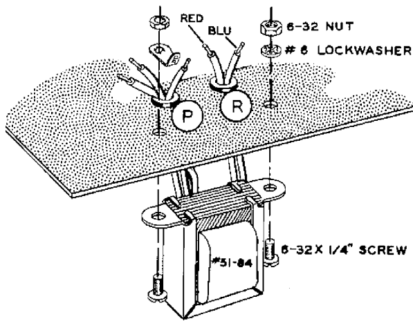
Detail 1F
