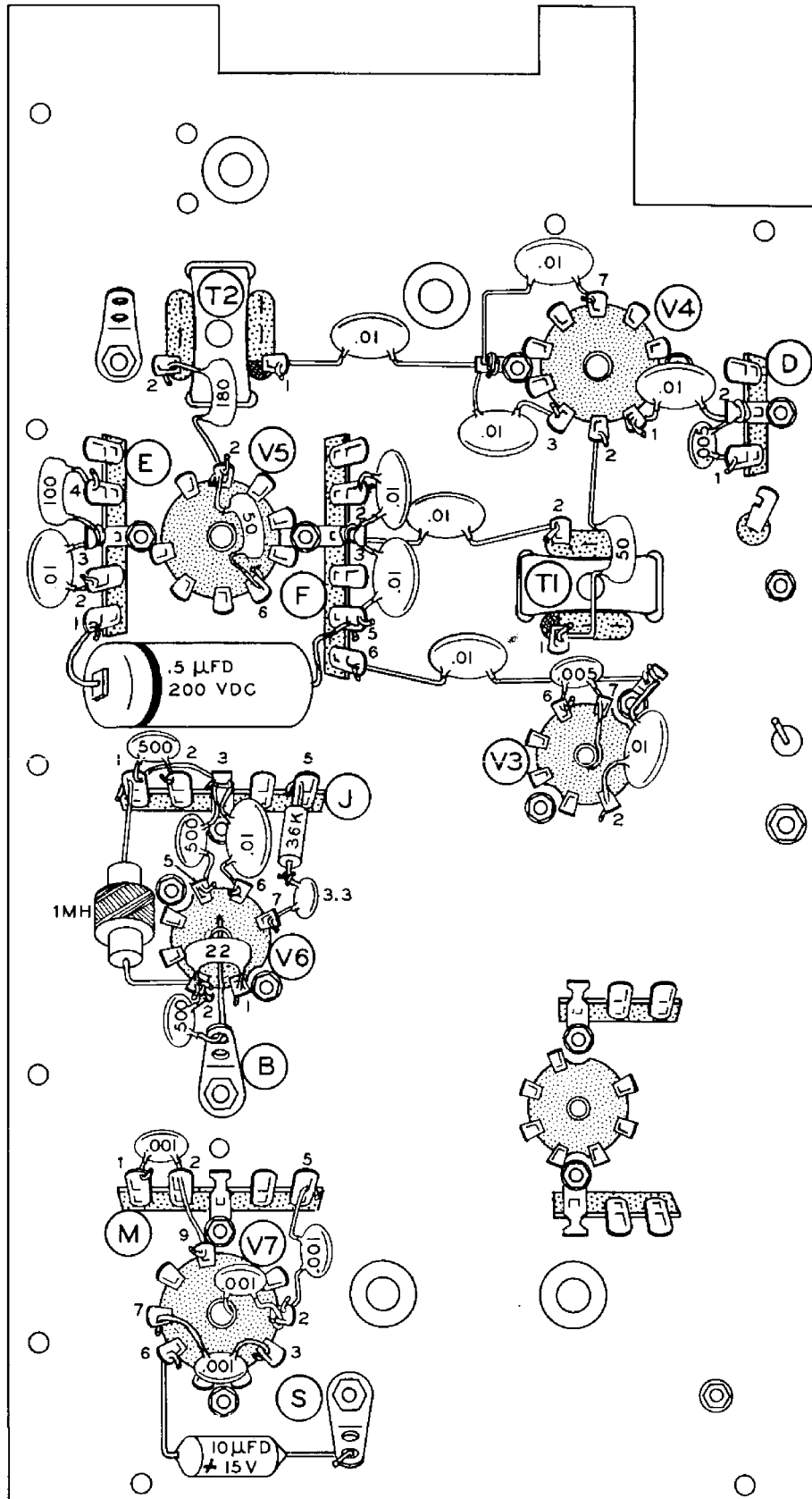
Pictorial 4
