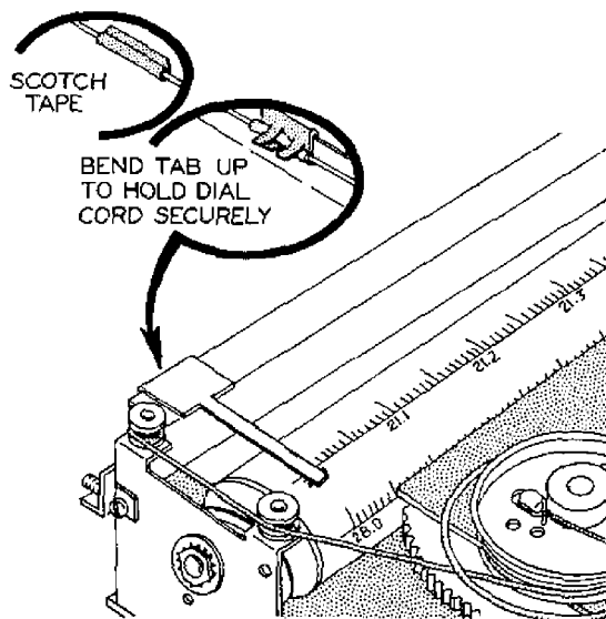
Detail 16A
