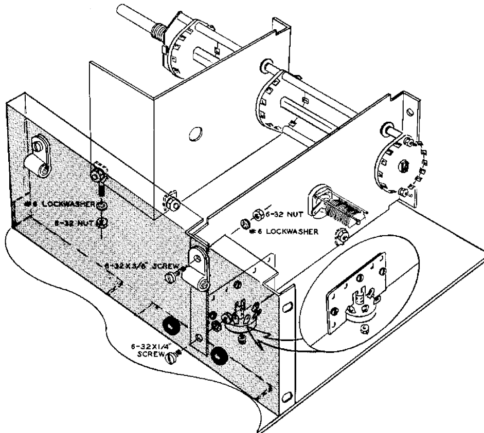
Pictorial 8
