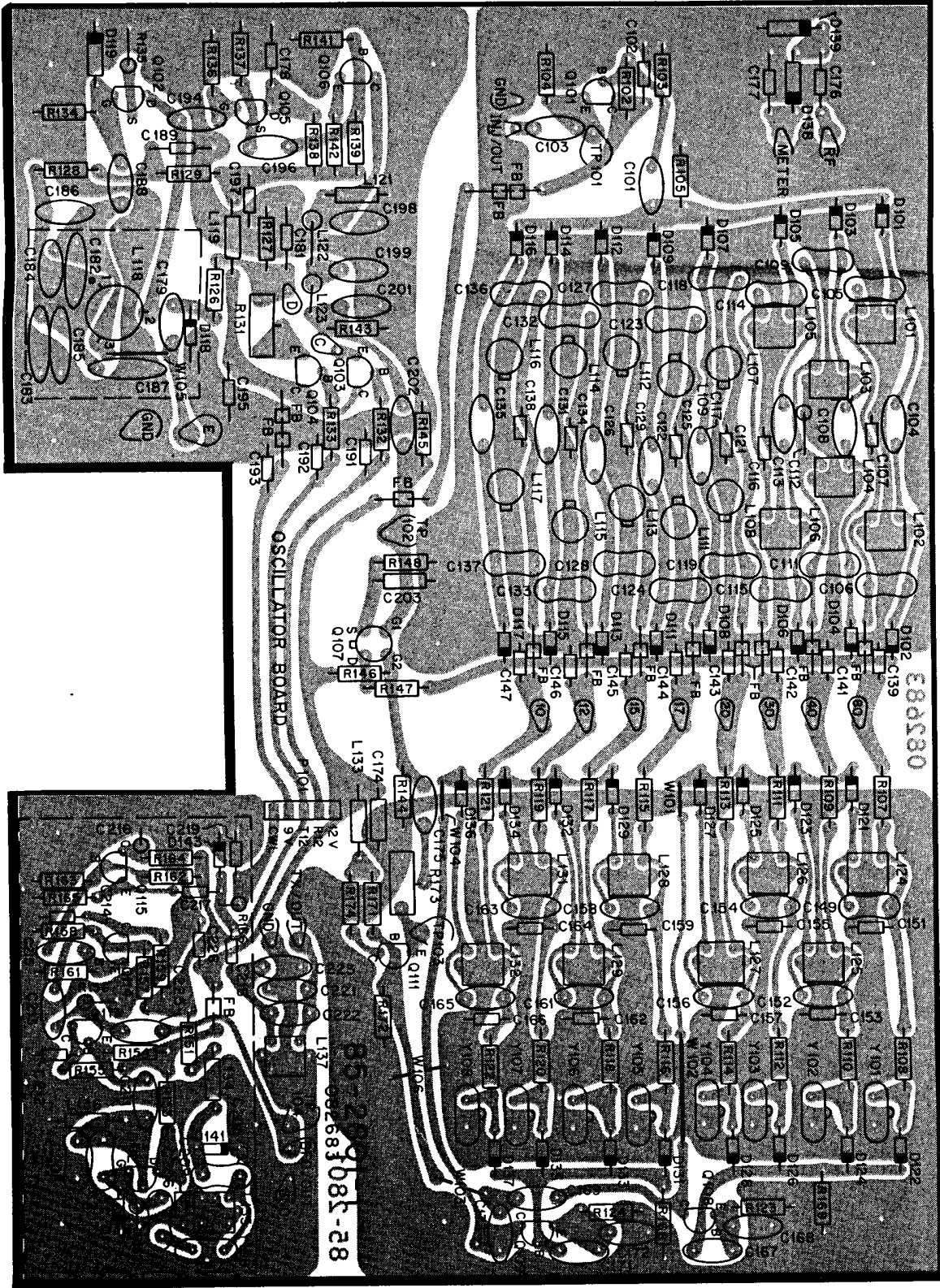
Oscillator Circuit Board (Shown from the component side.)
