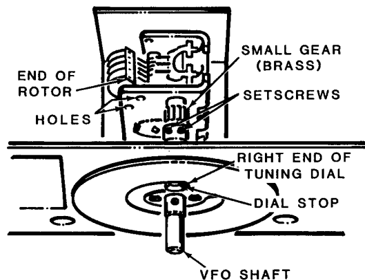
Detail 3-2C
