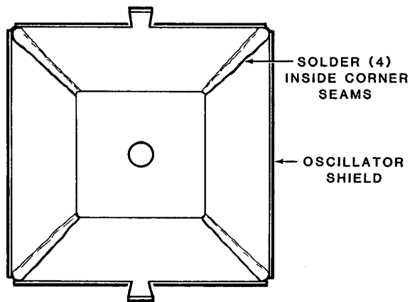
Detail 1-6A
