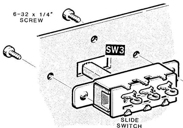
Detail 3-12A
