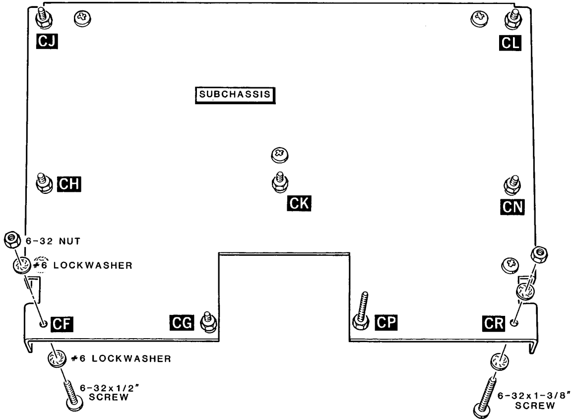
PICTORIAL 3-4
