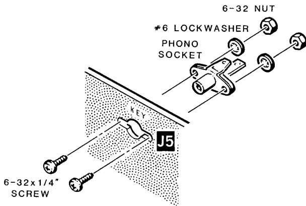
Detail 3-14C
