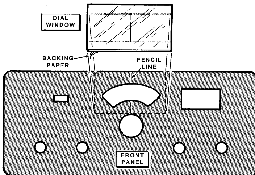
Detail 3-15A
