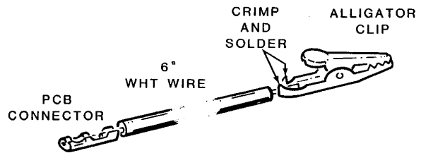
PICTORIAL 3-17
