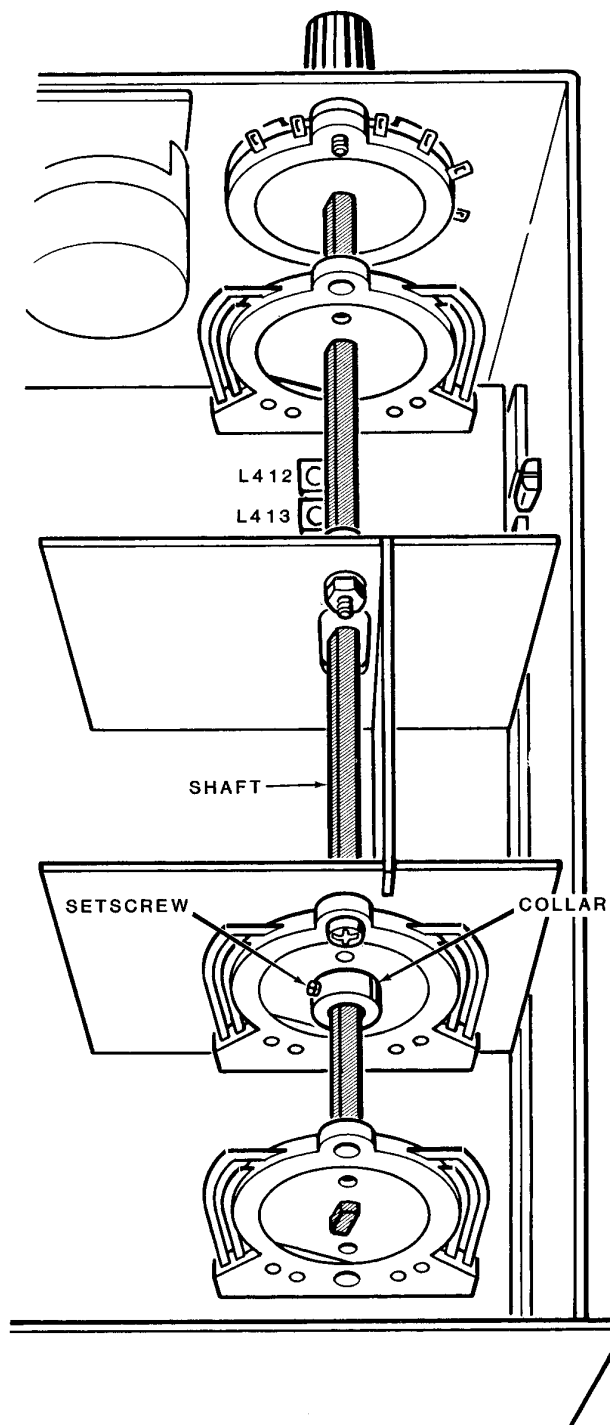
Detail 5-4A
