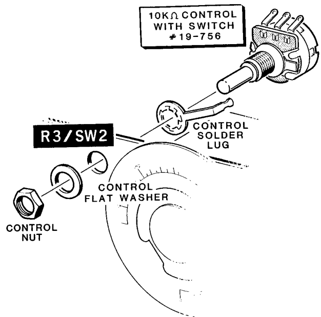
Detail 3-5C
