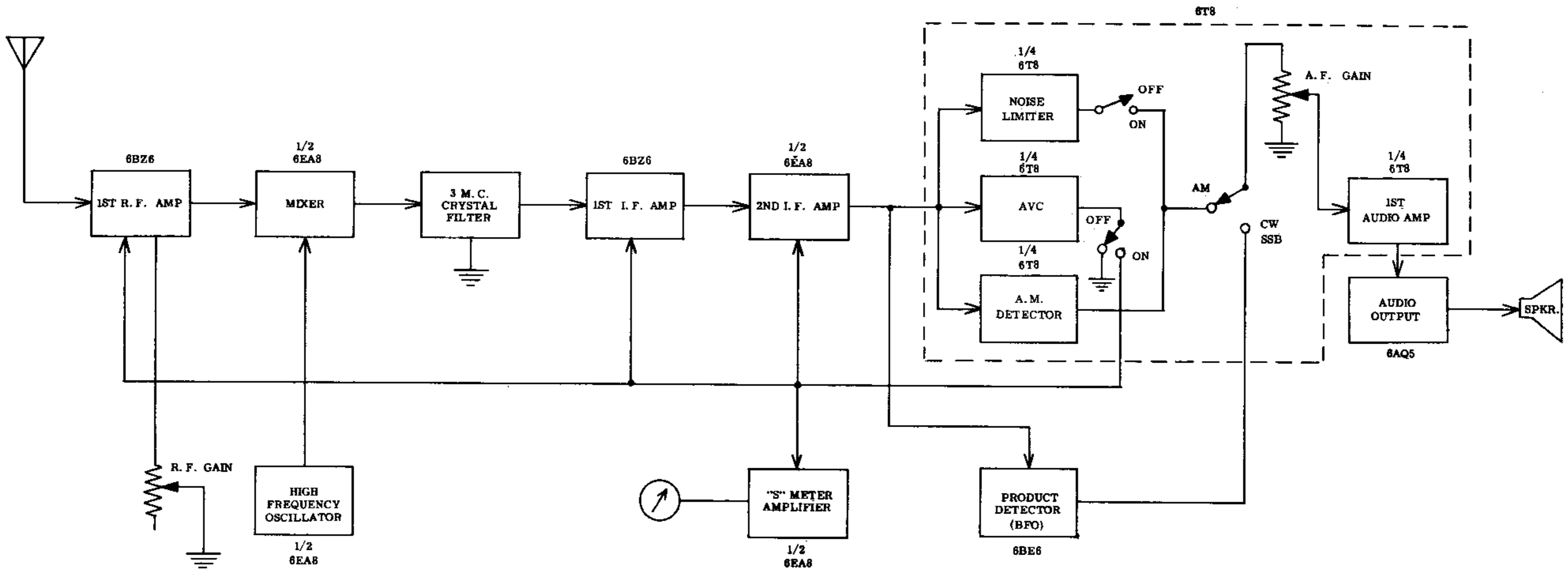
BLOCK DIAGRAM
