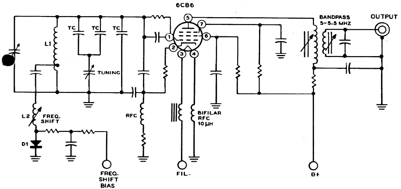
LMO SCHEMATIC
