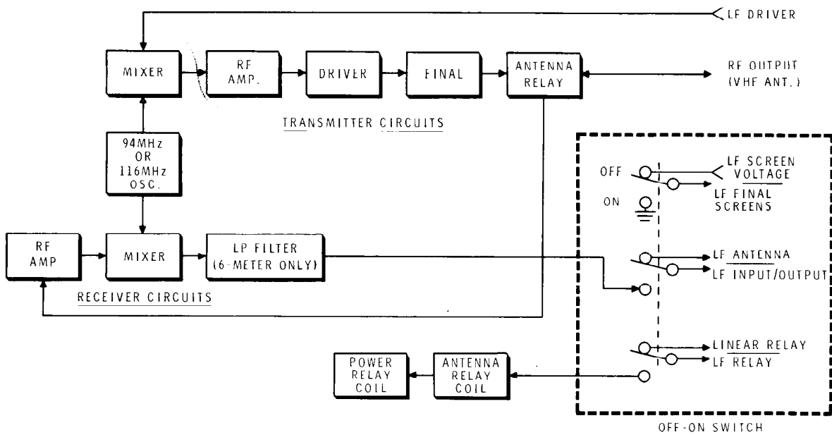
Figure 12-1 Block Diagram
