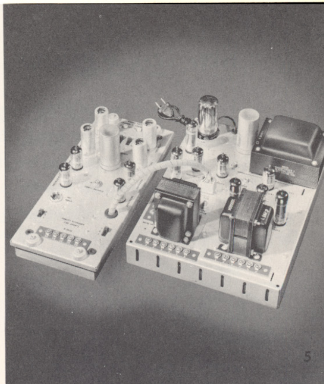
STEREO SET-UP (A+C+D)
