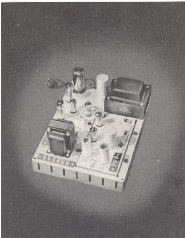
MONAURAL SET-UP (A+B)
