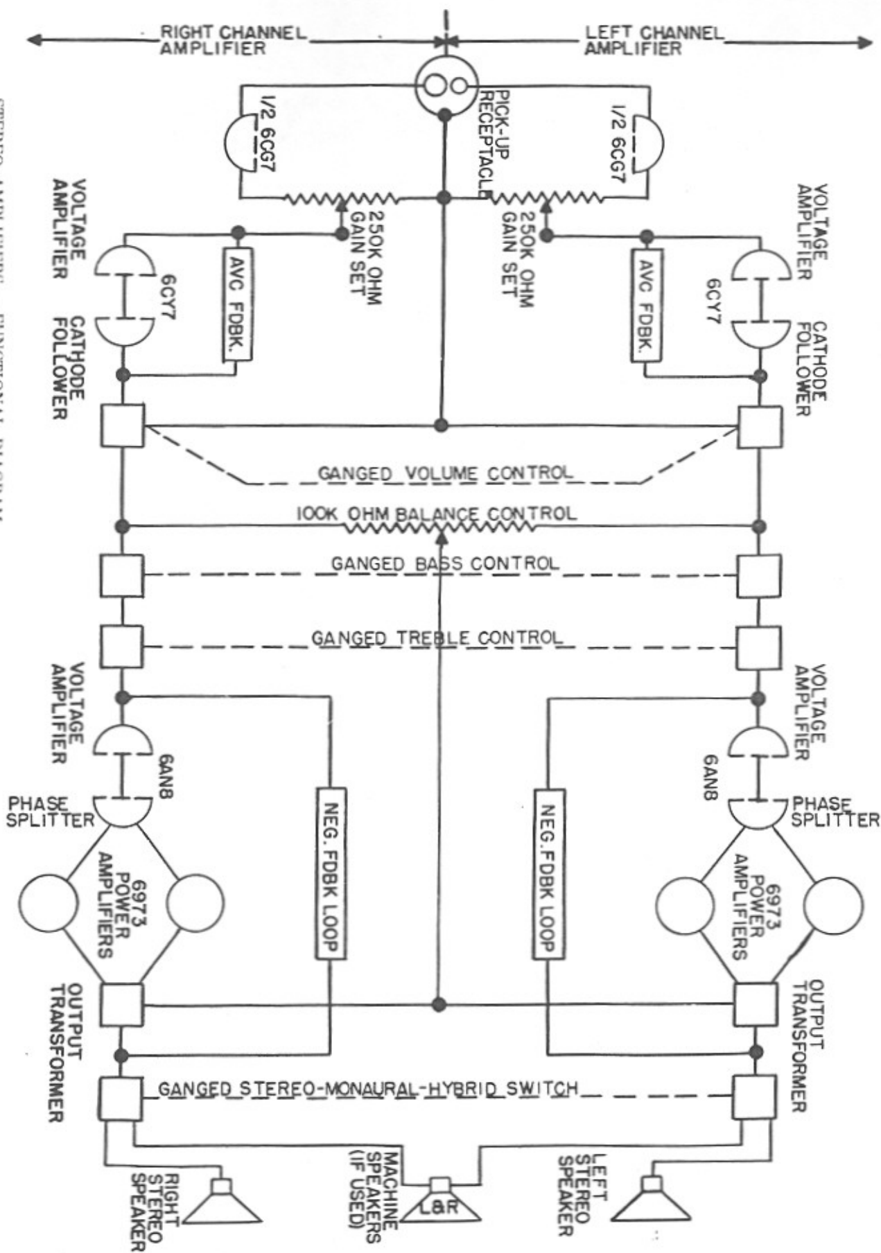
STEREO AMPLIFIERS — FUNCTIONAL DIAGRAM
