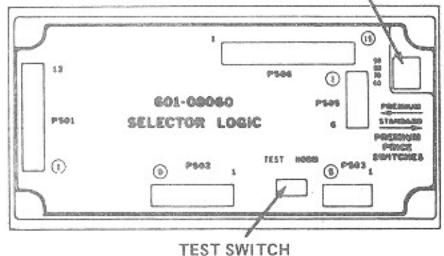
FIGURE 2-16. SWITCH LOCATIONS ON SELECTOR LOGIC MODULE
