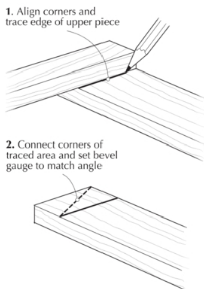
PIECES OF UNEQUAL WIDTH
