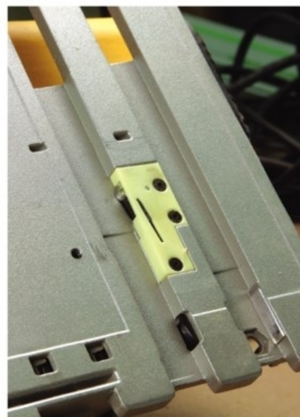
Spring to action. A spring-loaded roller locks the DeWalt saw to a DeWalt track. This is a great feature if you're using this saw as a panel-cutting tool.
