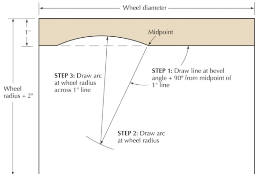
Jig layout. This shows the geometrical layout to produce a specific bevel angle. The shaded portion is the final jig.
