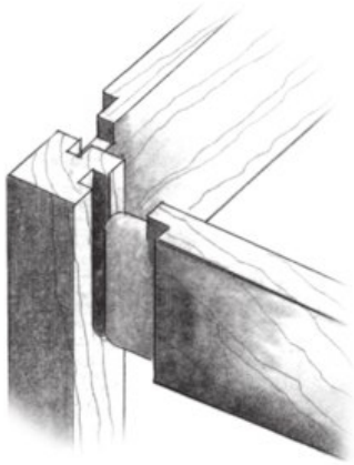
APRON TO BACK LEG JOINERY
