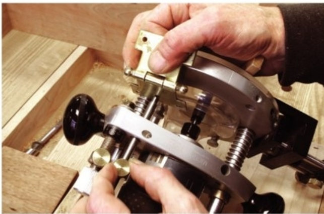
Better than measuring. Use a leaf of the hinge to set the depth stop on the plunge router. Set the bottom of the bit flush with the router base, then set the depth stop to the hinge. Plunge the router to the stop and you're set.
