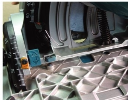
A tale of two levers. Flip a lever to bypass the 45° stop and cut at the maximum-cut angle of 48° – or push in the twin tabs to drop the saw to cut at a negative angle. These are two features that are unique to Makita's saw.
