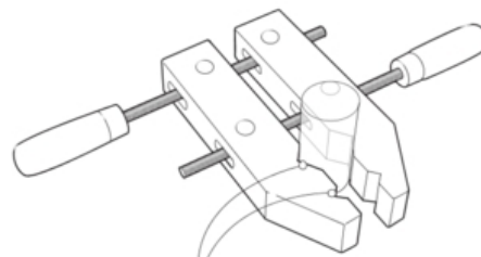
Notches hold short pieces on end for boring on drill press
