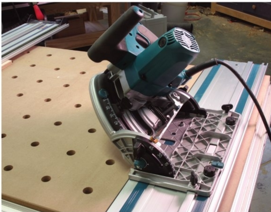
Stays on track. On the Makita, a small lever slides a catch into an undercut groove and does something that no other track saw can do – stay hooked to the track when all the weight is tilted.
