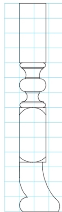
1 SQUARE = 1" FOOT PATTERN
