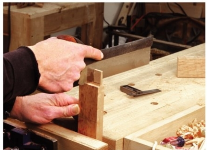
Faster by hand. Cutting the haunch by hand is faster than setting up to make these cuts by machine. Only the end of the haunch will be seen in the finished door, so this is a good place to practice making cuts by hand.
