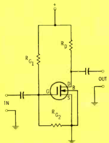
Fig. 5 Circuit employing enhancement MOSFET biased to operate in the type C mode (little source-to-drain current until gate potential is increased in positive direction). R_{G1} and R_{G2} form a bleeder circuit to supply turn-on bias to the gate. If you zero-bias the gate by connecting a jumper from gate to source, the source-to-drain current will be reduced to near zero, or about 1 microampere.
