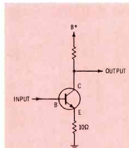
Fig. 1 Basic common-emitter circuit.
