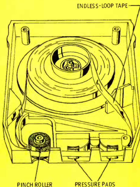
Fig. 1 Typical "stereo 8" auto tape-player cartridge. ¼-inch wide tape is pulled from and rewound on same reel in this closed-loop system, which has built-in pinch roller. The pressure pad on left holds tape against playback head. The guide cover prevents the tape from rubbing together as it moves through its closed loop of travel.
