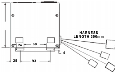
Overall Dimensions in mm
