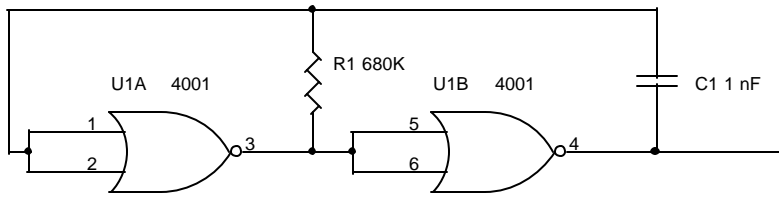
1 KHz Oscillator
