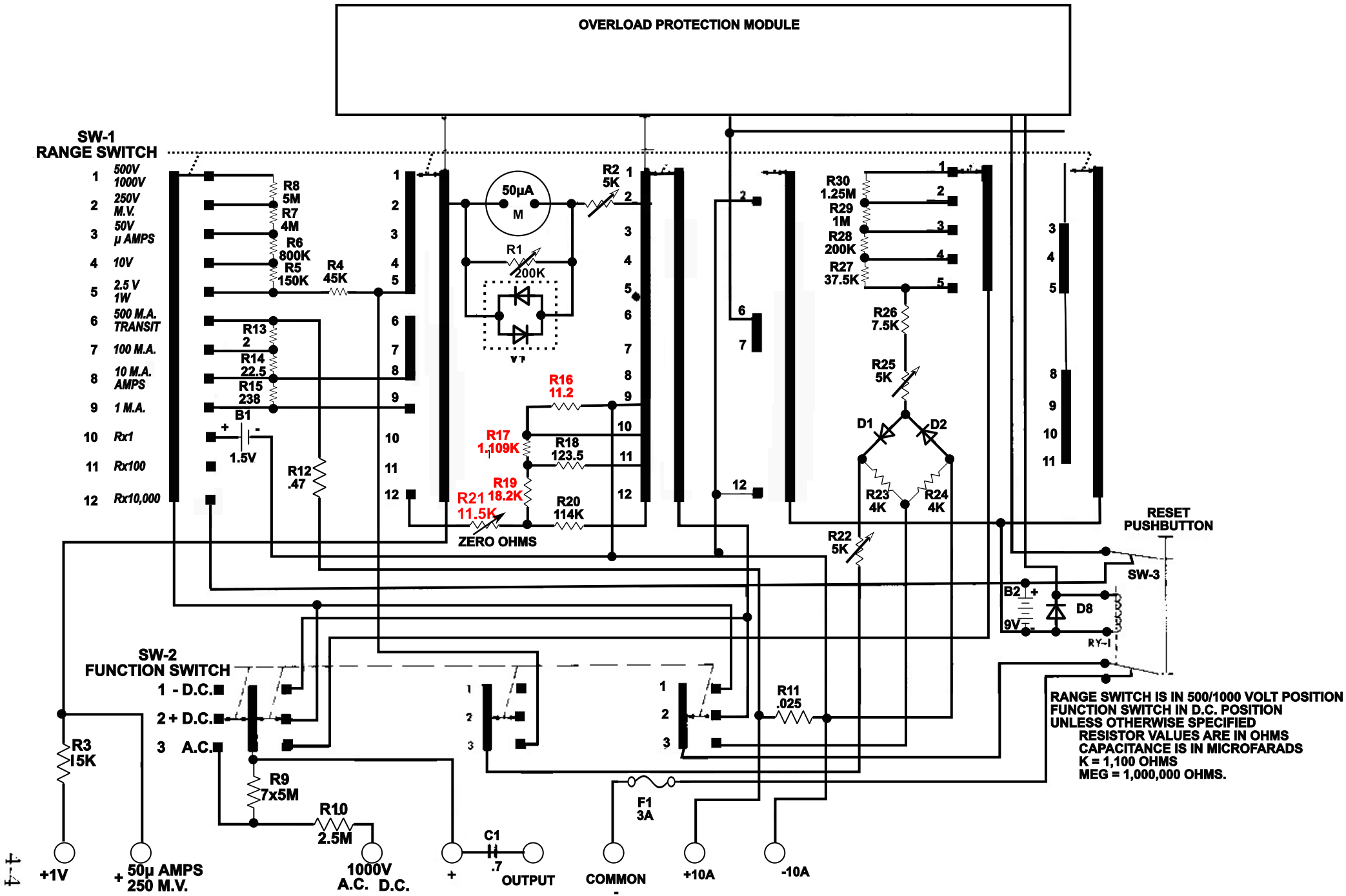
Figure 4-1. Simpson 260-6P, Schematic Diagram
