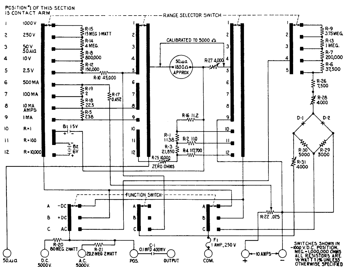
OVERALL SCHEMATIC, SIMPSON VOLT-OHM-MILLIAMMETER 260 ® SERIES III
